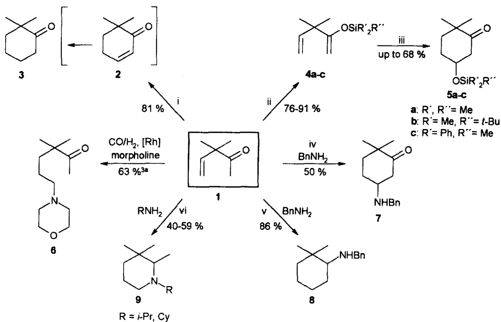
Scheme 2 7 . i: CO/H 2 (1:1), 80 bar, 100 °C, 3 d, CH 2 Cl 2 , [Rh(cod)Cl] 2 , p -TsOH·H 2 O (10 mol %); ii: a) 8 LDA, THF, -78 °C b) R' 2 R''SiCl, -78 °C to 20 °C; iii: CO/H 2 (1:1), 80 bar, 90 °C, 3 d, CH 2 Cl 2 , [Rh(cod)Cl] 2 ; iv: CO/H 2 (1:2), 30 bar, 60 °C, 3 d, benzylamine, dioxane, Rh(CO) 2 (acac), BIPHEPHOS 9 ; v and vi: CO/H 2 (1:2), 90 bar, 120 °C, 3 d, benzylamine or RNH 2 (R = i -Pr, Cy), dioxane, [Rh(cod)Cl] 2 , P(OPh) 3 .
